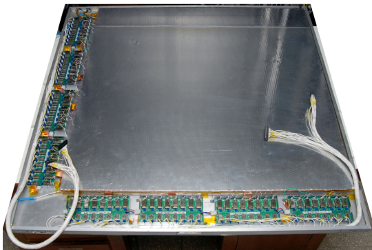
Fully assembled large area glass RPC (1 m \times 1 m)
